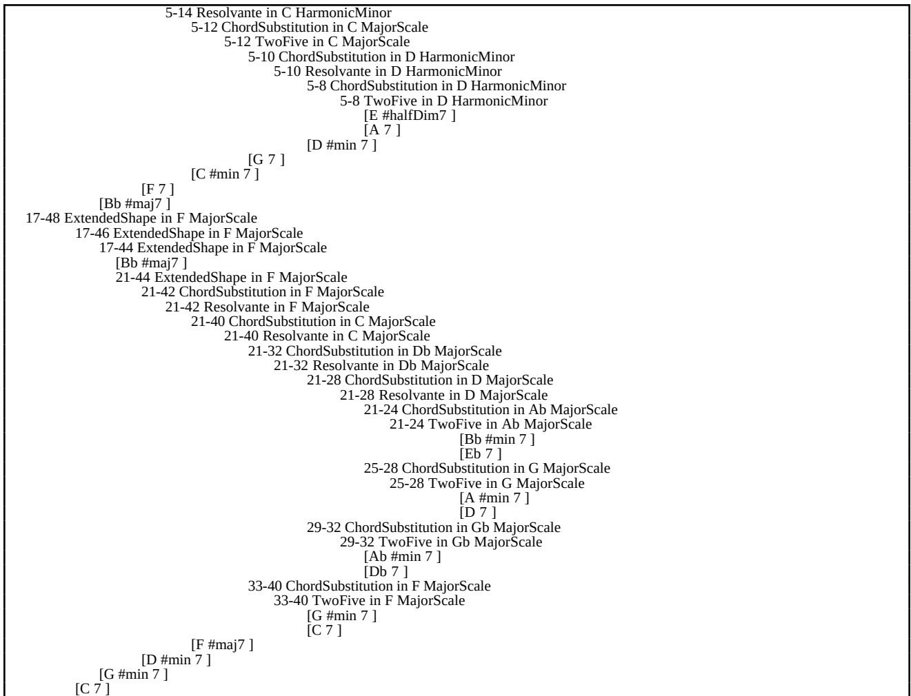
Figure 6. The complete analysis of the chord sequence of Figure 5.
