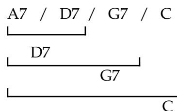
Figure 3. The hierarchical nature of the analysis of a group of chords.
