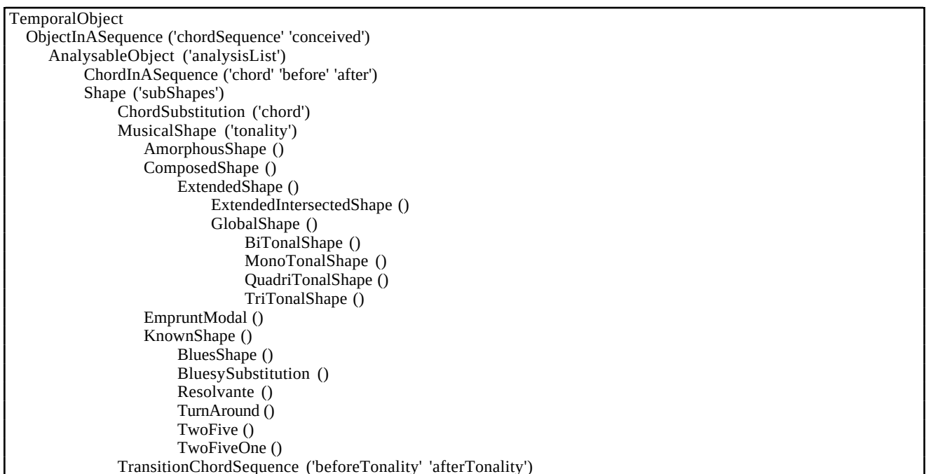
Figure 7. The various classes representing abstract analysis objects (attributes are between parenthesis).
